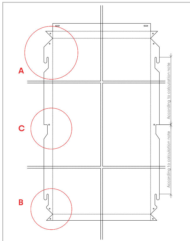
UNFOLDED CASSETTE
