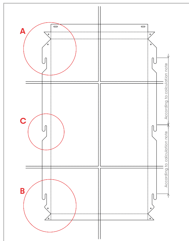
UNFOLDED CASSETTE
