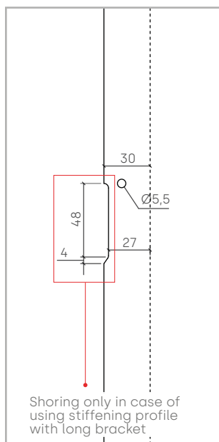
DETAIL C
