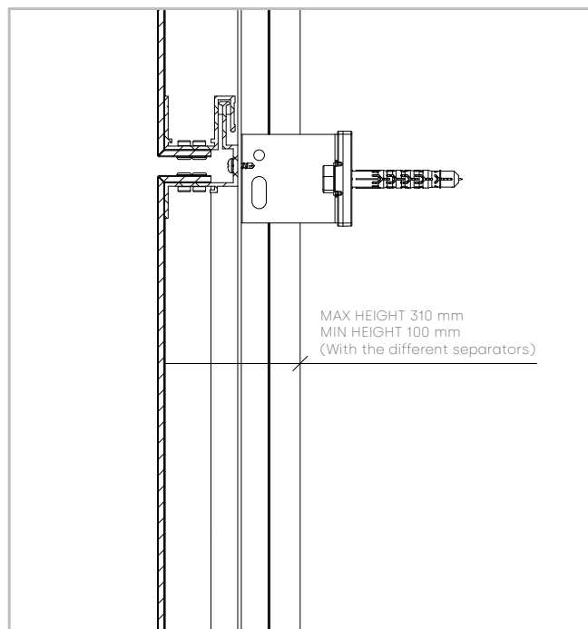
VERTICAL SECTION
