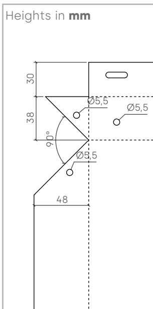
DETAIL A
