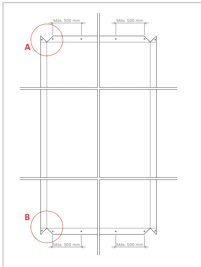
UNFOLDED CASSETTE
