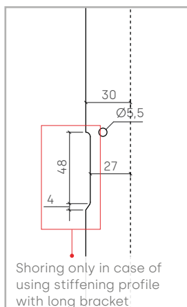
DETAIL C
