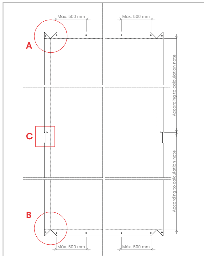
UNFOLDED CASSETTE
