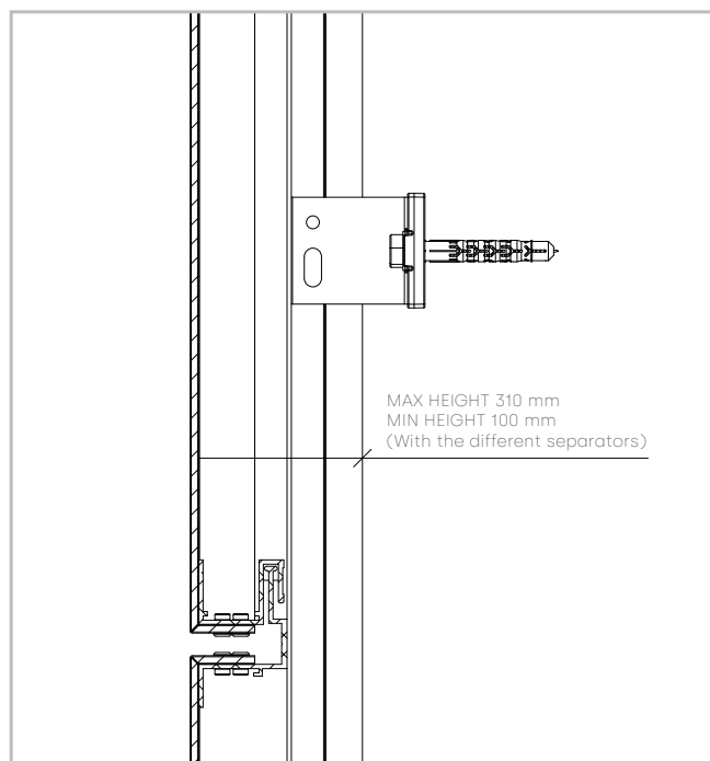
VERTICAL SECTION
