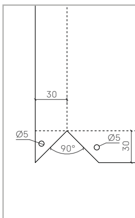
DETAIL B
